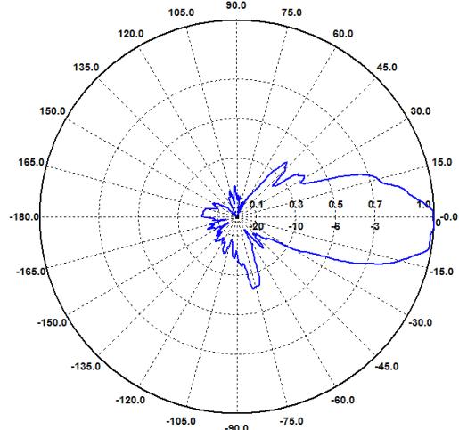
E-Ebene / E-Plane 3400 MHz
