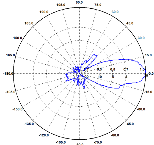
E-Ebene / E-Plane 3800 MHz
