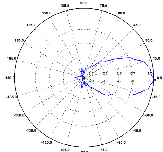
H-Ebene / H-Plane 1800 MHz
