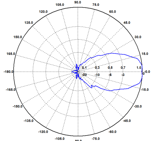
H-Ebene / H-Plane 1600 MHz
